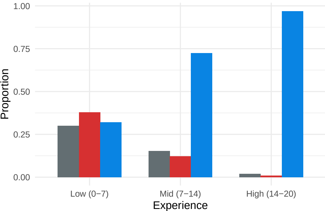
Observed proportions
